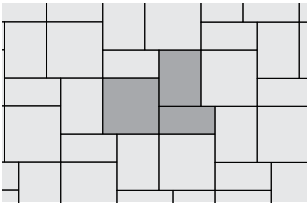
Arcana A - 44% 24" x 24", 33% 18" x 24", 23% 12" x 24"
