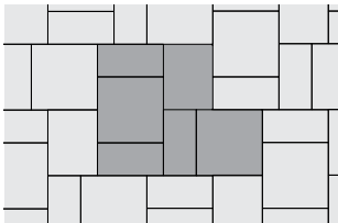
Arcana D - 46% 24" x 24", 18% 18" x 24", 36% 12" x 24"
