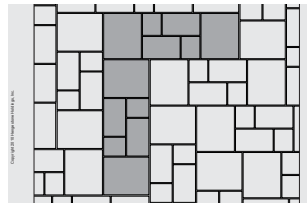
Thornbury B - 49% Large Rectangle, 34% Medium Rectangle, 17% Small Rectangle
