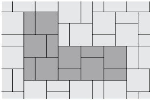
Natural Stone C - 67% 24" x 24", 33% 12" x 24"
