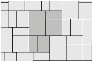
Natural Stone F - 34% 24" x 36", 24% 24" x 24", 18% 18" x 24", 24% 12" x 24"
